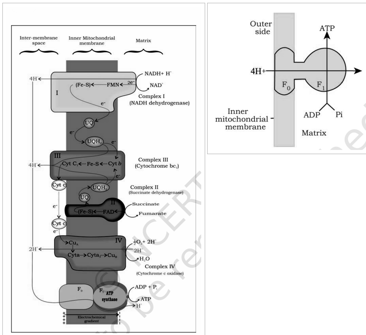
Fig. 12.4 - Electron Transport System (ETS). The carriers sit in the inner mitochondrial membrane between the inter-membrane space and the matrix . At Complex I (NADH dehydrogenase) , \text{NADH} + \text{H}^+ is oxidised to \text{NAD}^+ , handing 2e^- to \text{FMN} and the \text{Fe-S} centres while 4\text{H}^+ are pumped out; the electrons pass to \text{UQ} , which becomes \text{UQH}_2 . At Complex II (Succinate dehydrogenase) , succinate is oxidised to fumarate via \text{FAD} and \text{Fe-S} , also reducing \text{UQ} . Complex III (Cytochrome \text{bc}_1 ) passes electrons through \text{Cyt } b , \text{Fe-S} and \text{Cyt } c_1 to \text{Cyt } c , pumping a further 4\text{H}^+ . Complex IV (Cytochrome c oxidase) carries them through \text{Cu}_A , \text{Cyt } a , \text{Cyt } a_3 and \text{Cu}_B , reducing \text{O}_2 with 2\text{H}^+ to \text{H}_2\text{O} . The protons return through \text{F}_0 and drive \text{F}_1 ATP synthase down the electrochemical gradient , making ATP from \text{ADP} + \text{P}_i .
